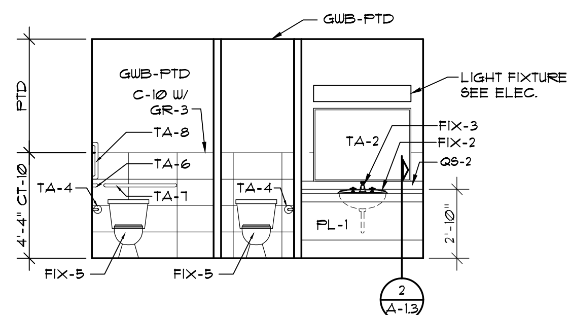
WOMEN 117 INTERIOR ELEVATION 3 A-13 SCALE: 1/4" = 1'-0"
