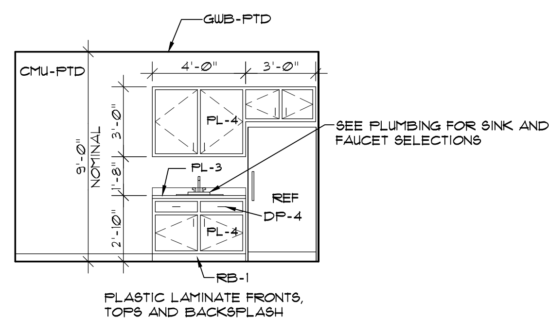
TECH BREAK 130 INTERIOR ELEVATION SCALE: 1/4" = 1'-0"
