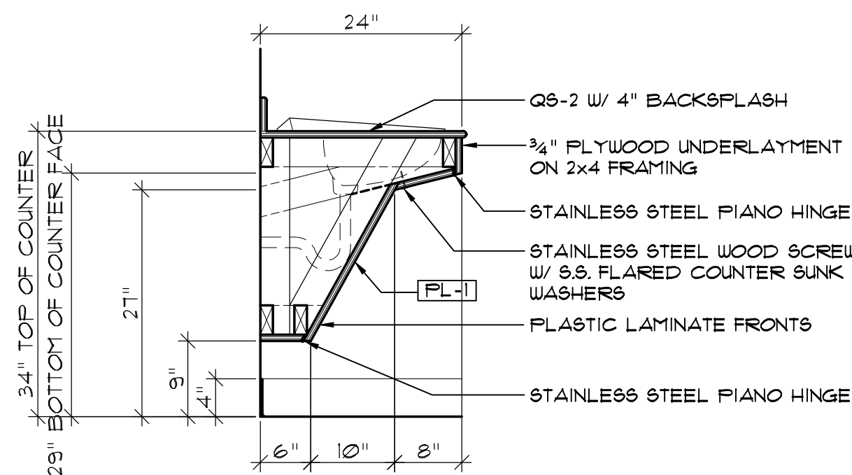
2 A-1.3 H.C. VANITY DETAIL SCALE: 3/4" = 1'-0"
