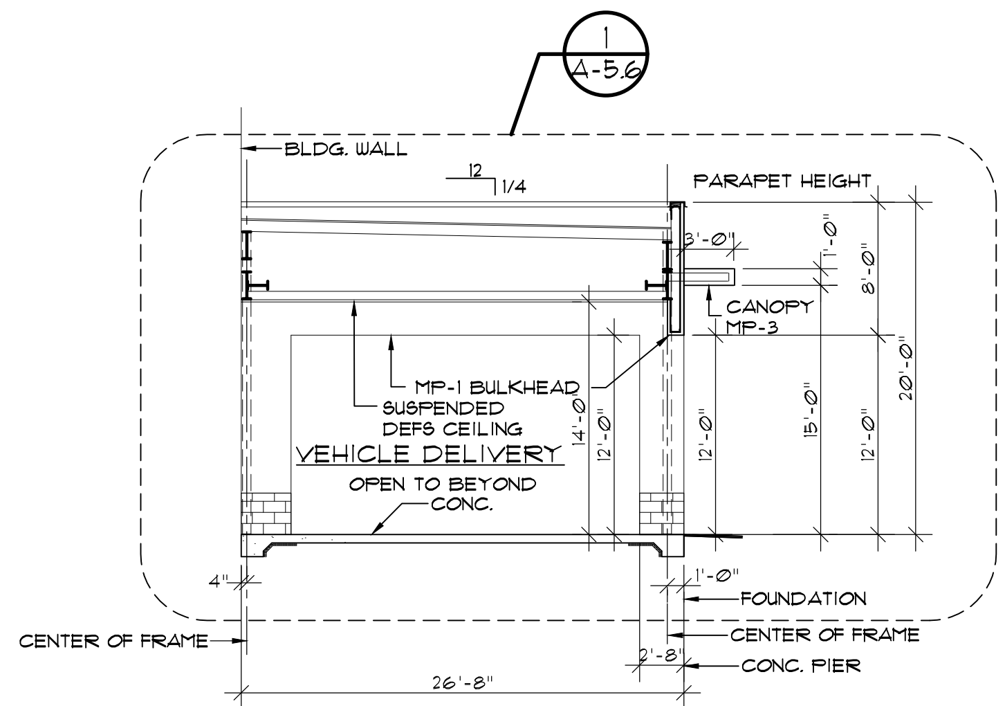
5 A-5 SCHEMATIC VEHICAL DELIVERY SECTION SCALE: 1/8" = 1'-0"
