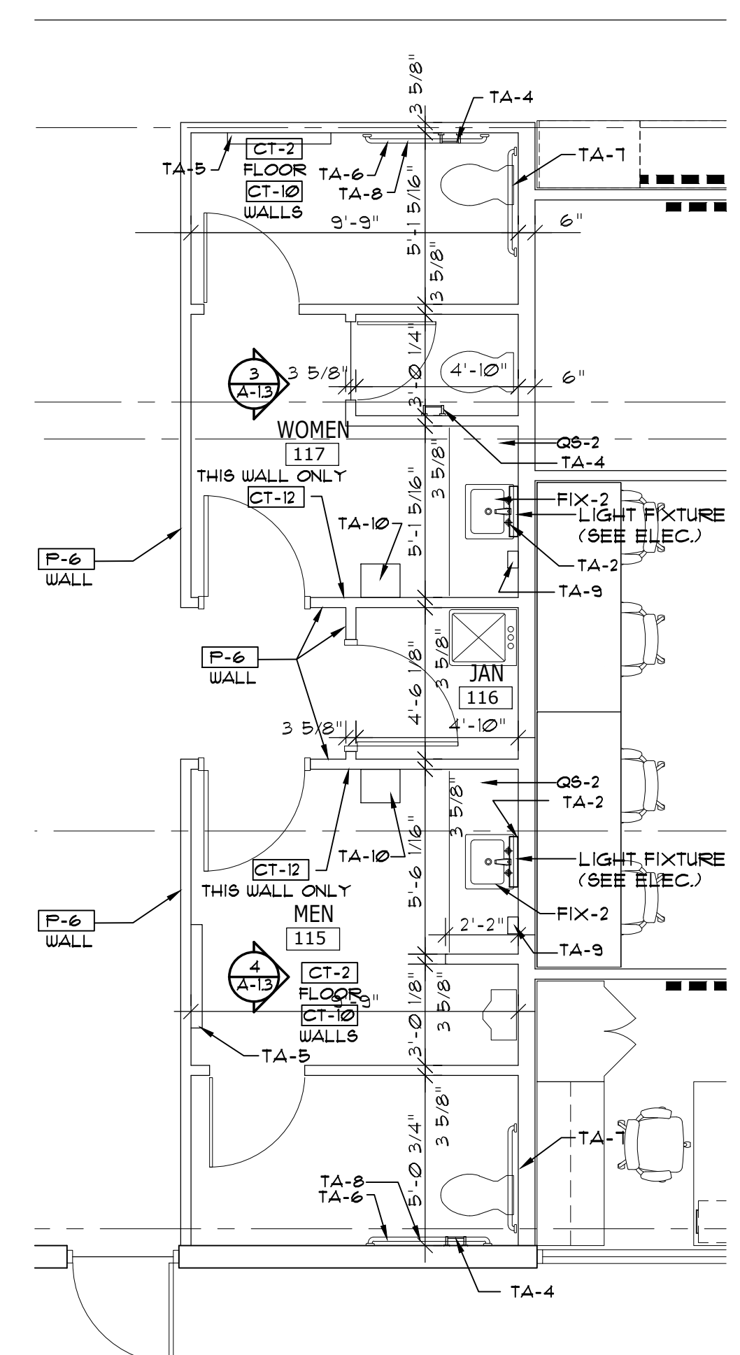
MEN 115 & WOMEN 117 TOILET PLAN DETAIL SCALE: 1/4" = 1'-0"
