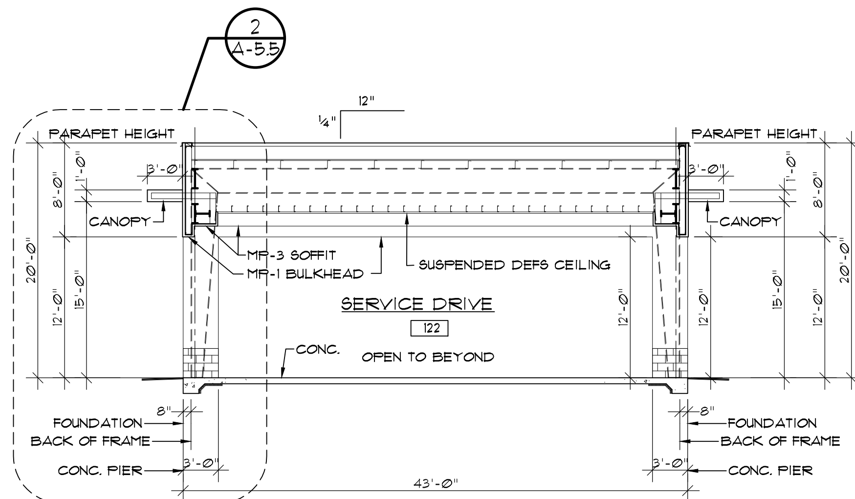
2 A-5.5 SCHEMATIC SERVICE DRIVE SECTION SCALE: 1/8" = 1'-0"
