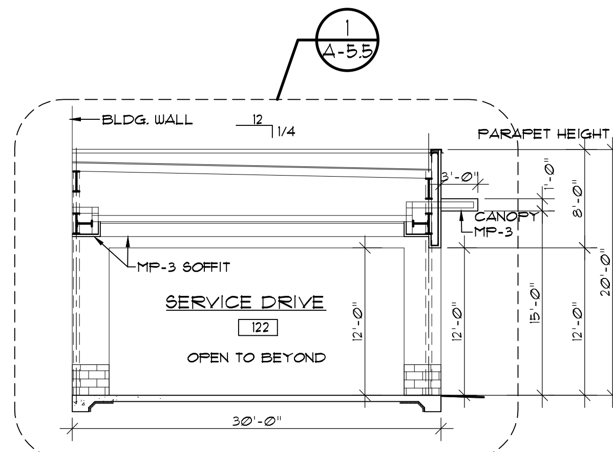
3 A-5 SCHEMATIC SERVICE DRIVE SECTION SCALE: 1/8" = 1'-0"
