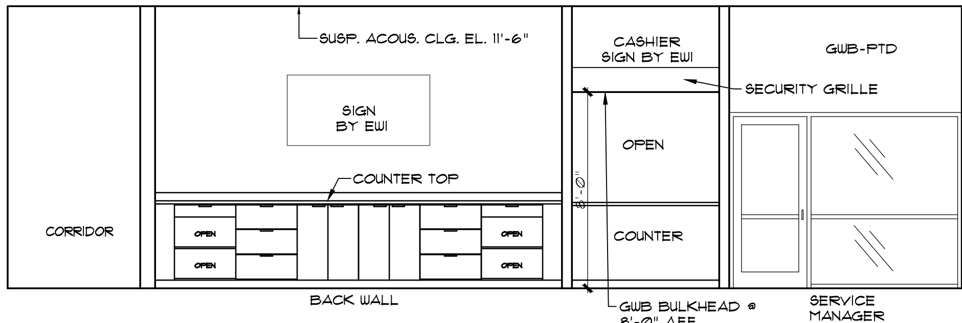
2 A-7.1 INTERIOR ELEVATION SCALE: 1/4"=1'-0"
