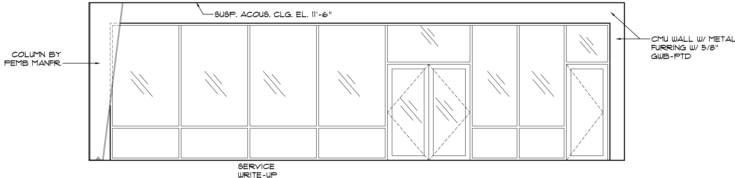
3 A-7.1 INTERIOR ELEVATION SCALE: 1/4"=1'-0"
