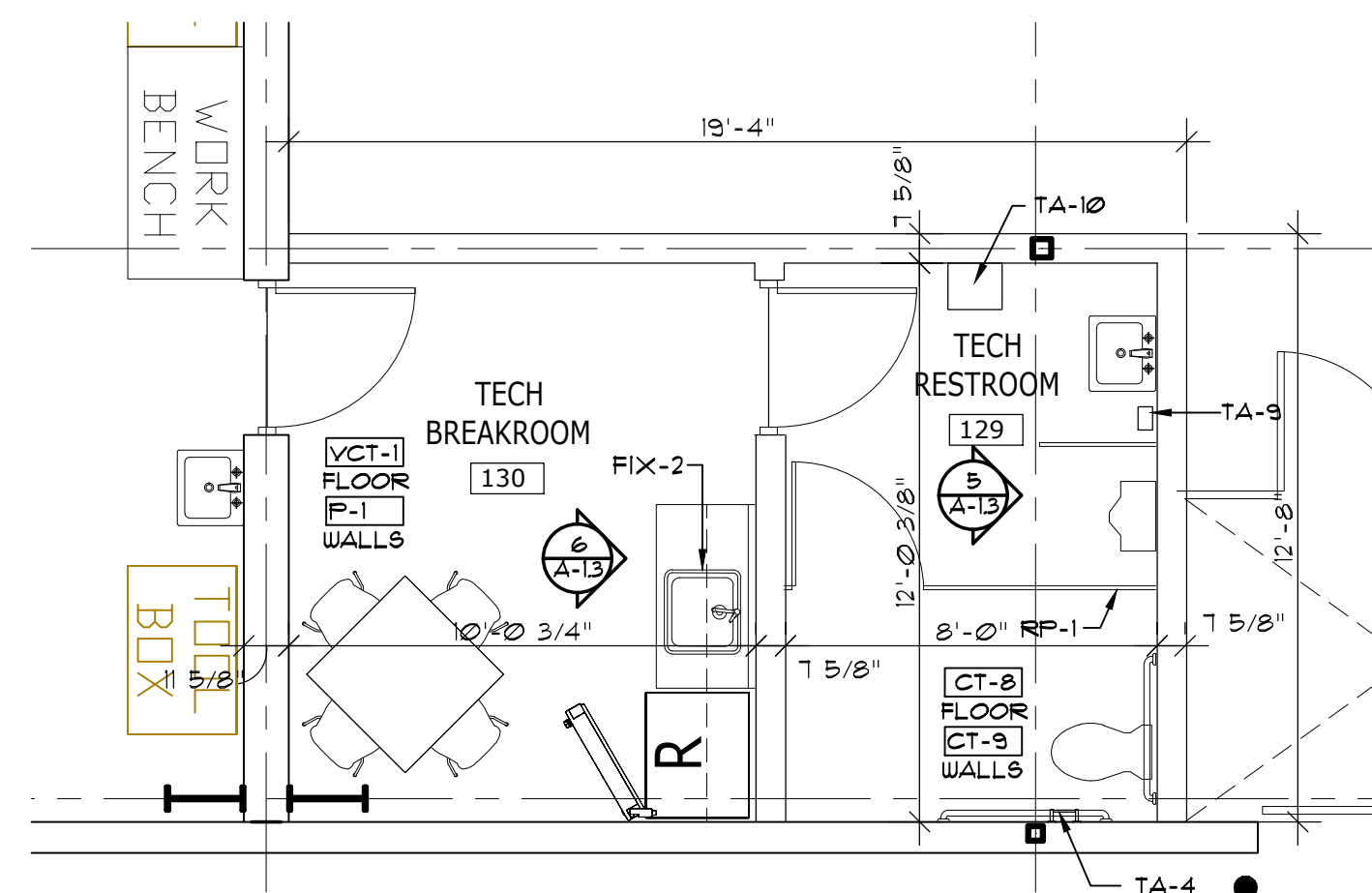
TECH BREAKROOM TECH TOILET PLAN DETAIL SCALE: 1/4" = 1'-0"
