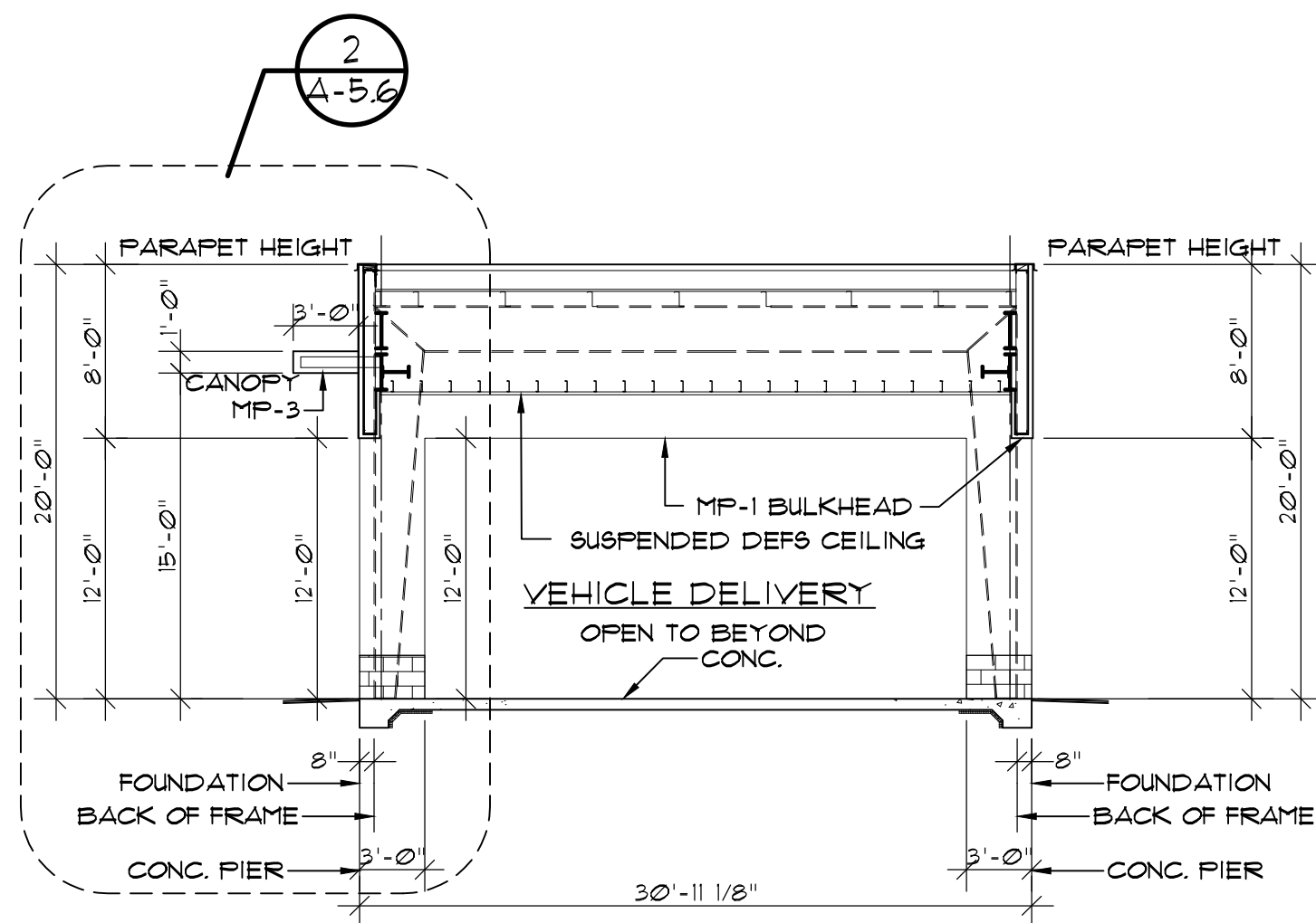
4 A-5 SCHEMATIC VEHICAL DELIVERY SECTION SCALE: 1/8" = 1'-0"
