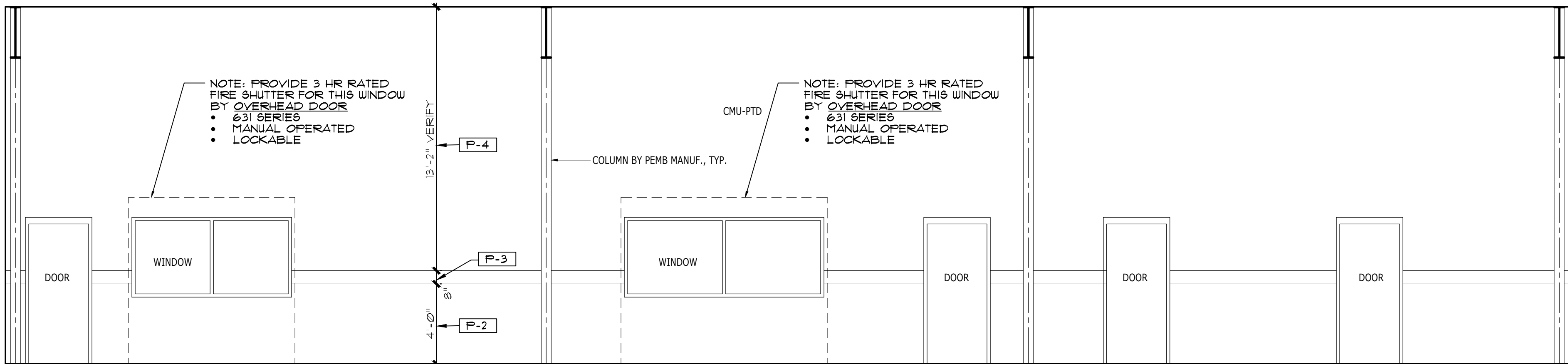
1 A-7.1 INTERIOR ELEVATION SCALE: 1/4"=1'-0"
