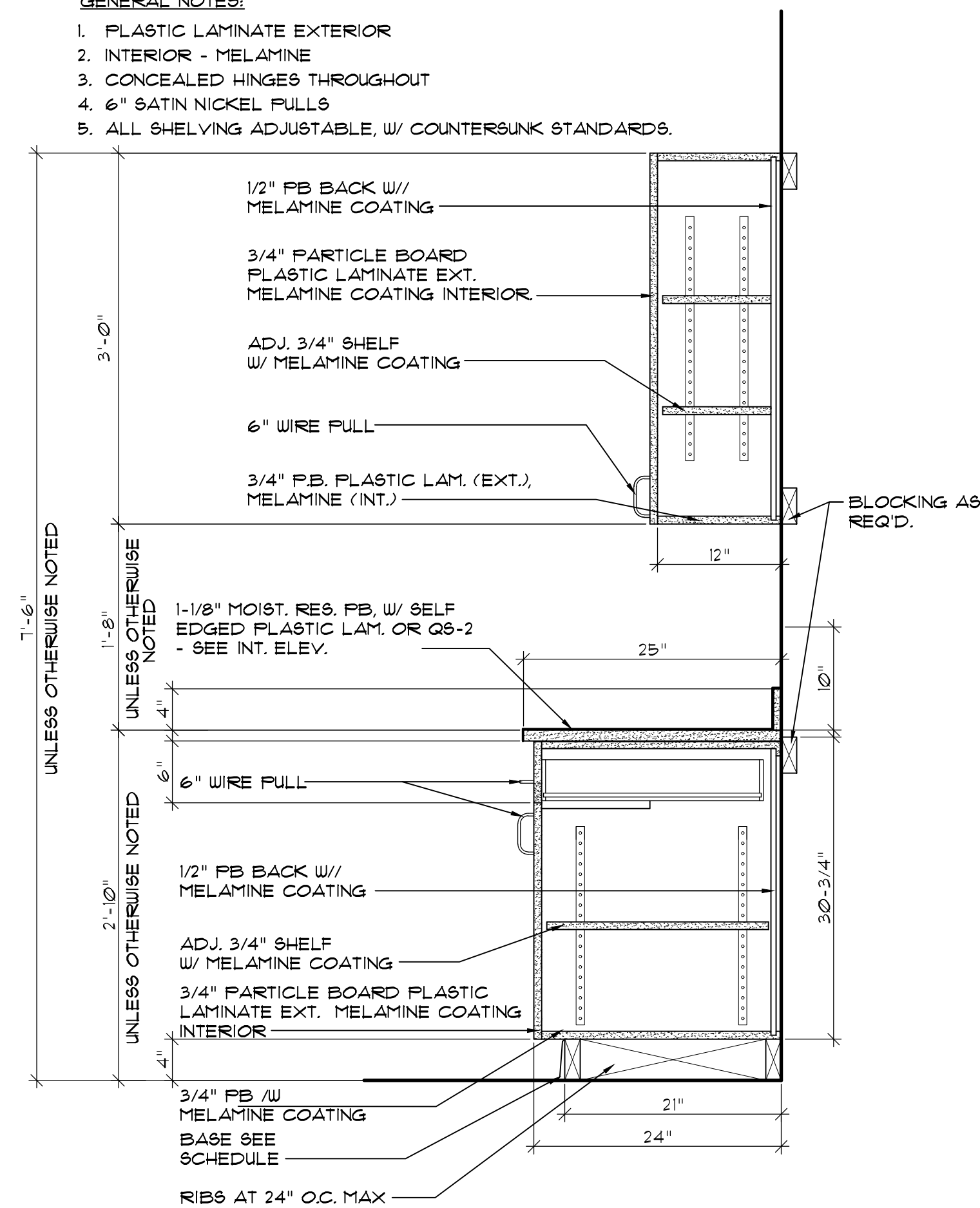
1 TYP. CABINET DETAIL A-1.3 SCALE: 1"=1'-0"
