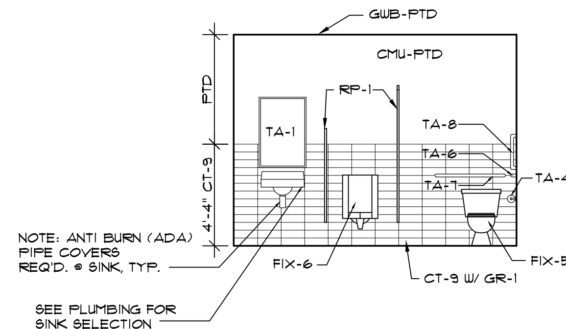
TECH RESTROOM 129 INTERIOR ELEVATION 5 A-13 SCALE: 1/4" = 1'-0"
