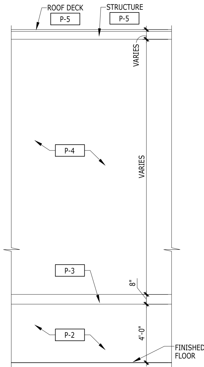
SERVICE BAY WALL ELEVATION
