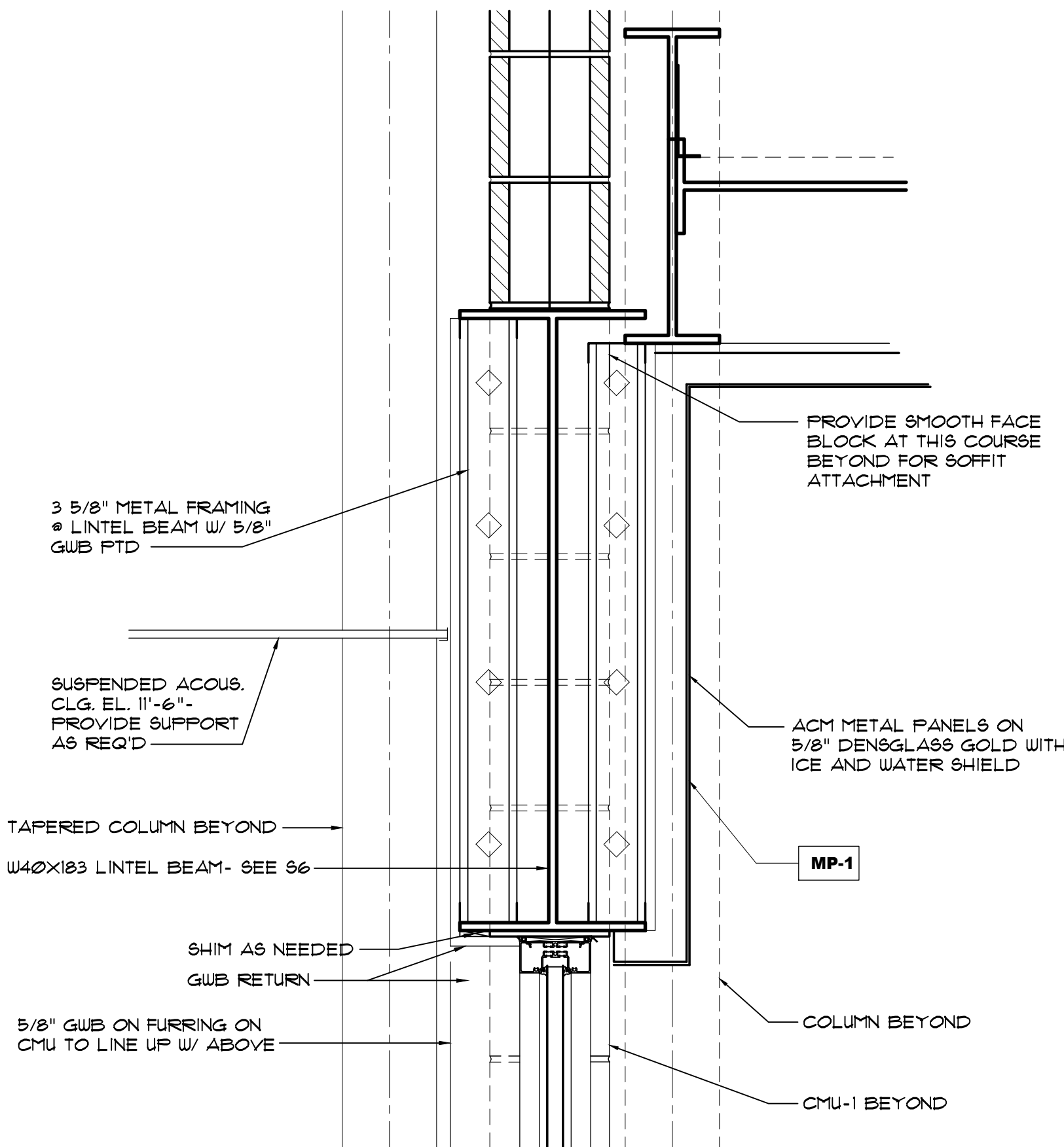
4 A-7.1 DETAIL @ W-BEAM LINTEL SCALE: 1/2"=1'-0"
