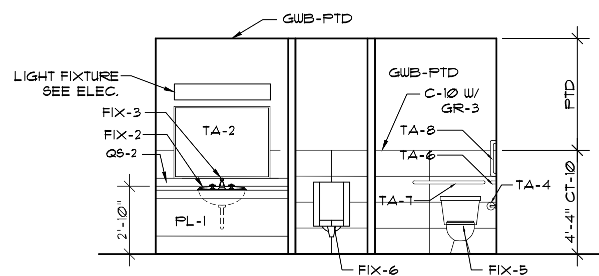
MEN 115 INTERIOR ELEVATION SCALE: 1/4" = 1'-0"
