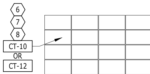
RESTROOMS - STACKED BOND WALL TILE PATTERN
